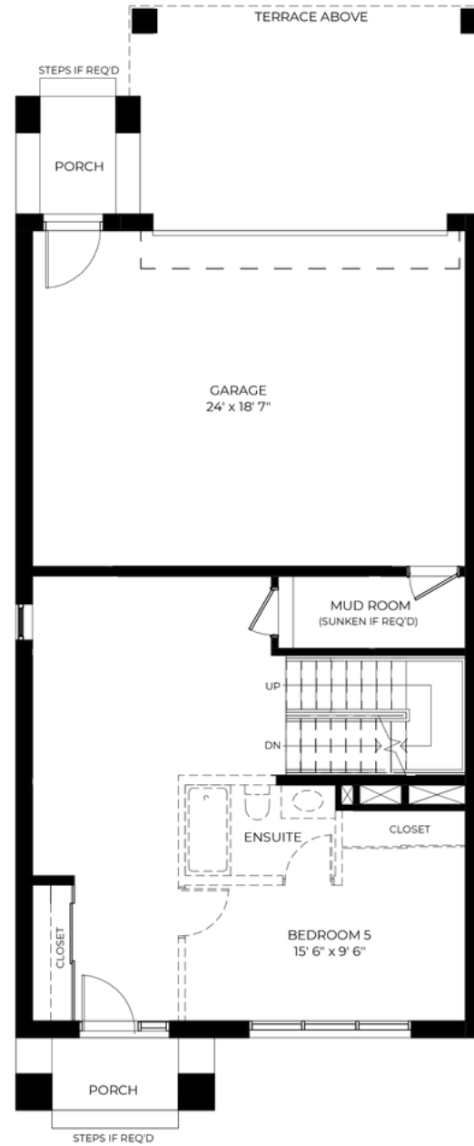
GROUND FLOOR
