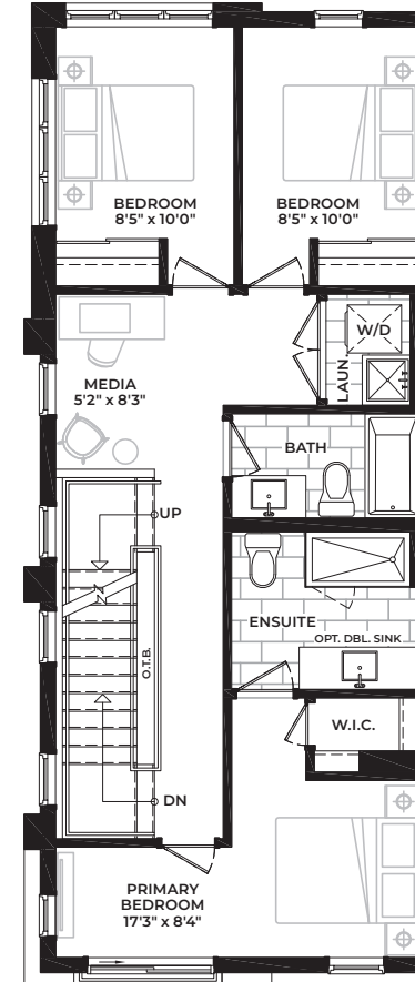
C1 Corner End THIRD FLOOR
