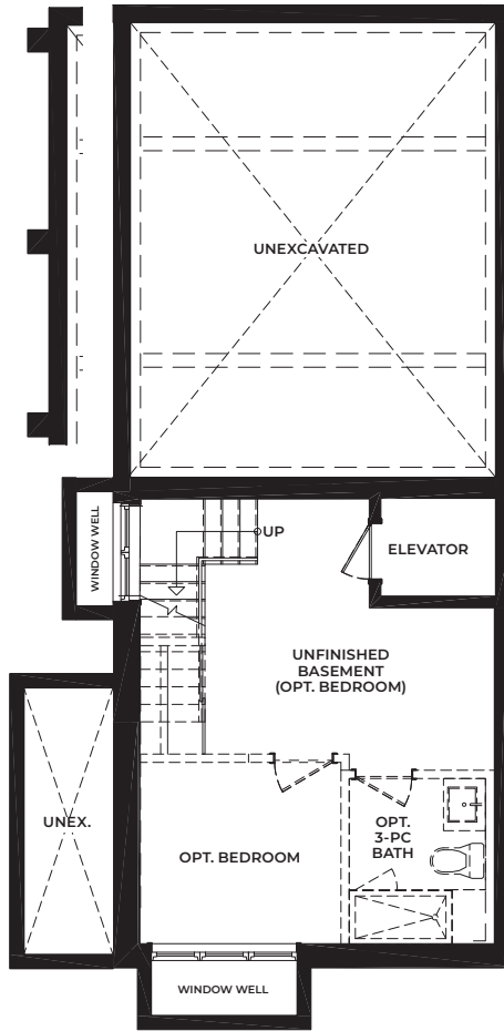
C1 Corner End Opt. Elevator & Opt. Bedroom BASEMENT
