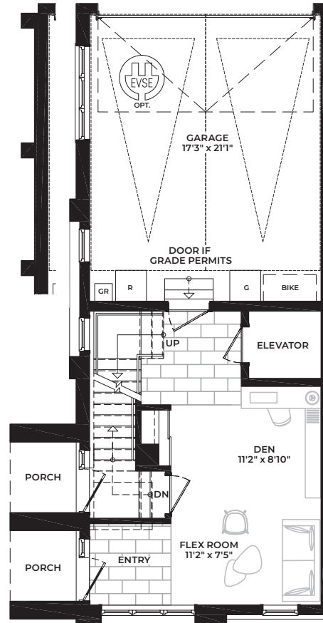
C1 Corner End Opt. Elevator & Opt. Bedroom GROUND FLOOR
