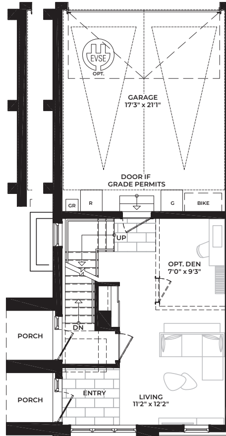
C1 Corner End GROUND FLOOR
