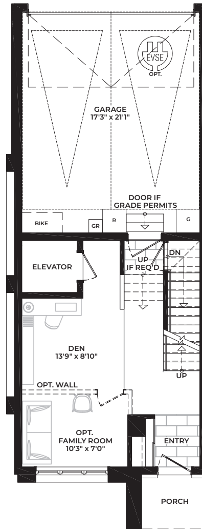
B1 End Opt. Elevator GROUND FLOOR
