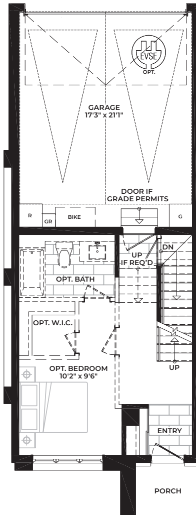
B1 End Opt. Bedroom GROUND FLOOR
